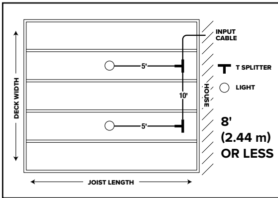
EXAMPLE OF A 2 ROW LIGHT INSTALLATION FOR JOISTS BETWEEN 9' AND 12' (2.76 - 3.65 m)
