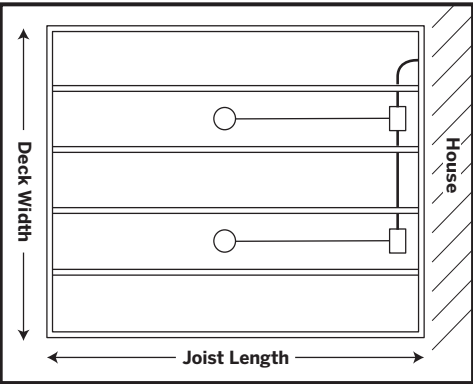
EXAMPLE OF A 2 ROW LIGHT INSTALLATION FOR JOISTS BETWEEN 9' AND 12' (2.76 - 3.65 M)
